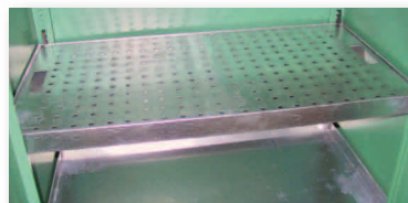
Galvanized shelves with retention tray and drainer
